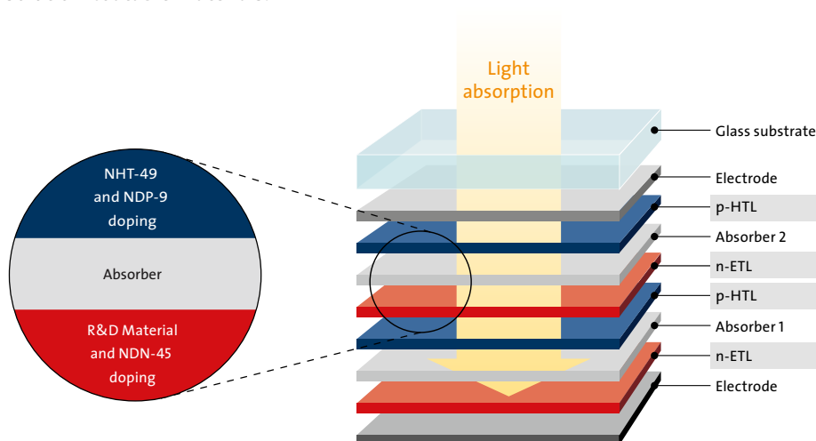
Organic Solar Cell with Novaled technology and materials
